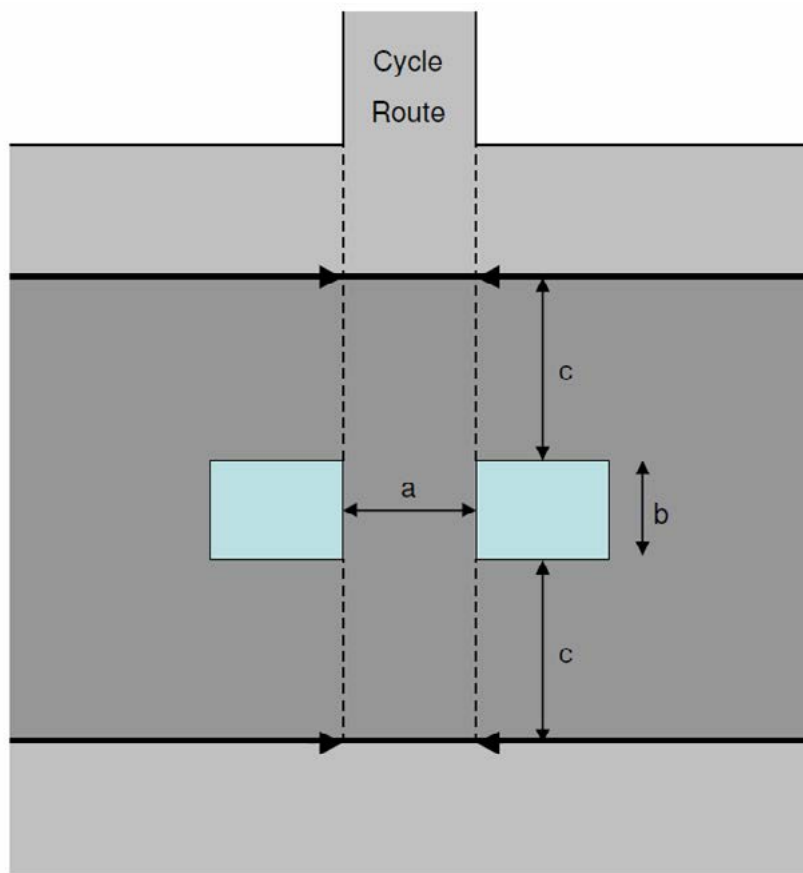
Figure 10 Cycle crossing preferred layout
