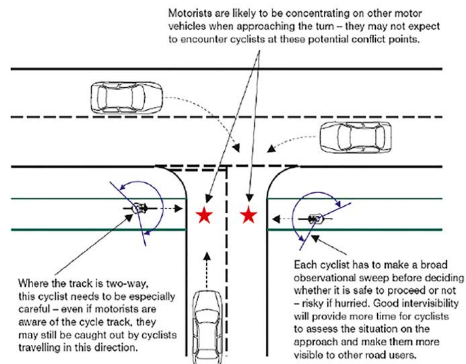
Figure 8 Intervisibility issues for 2-way cycle tracks at road junctions (Source: Superseded Local Transport Note 1/12 Shared use routes for pedestrians and cyclists )
