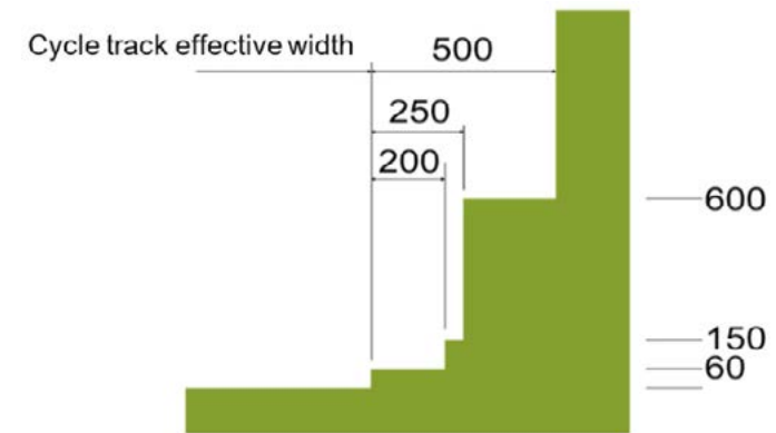
Diagram showing additional width at fixed objects based on LTN 1/20 table 5-3
